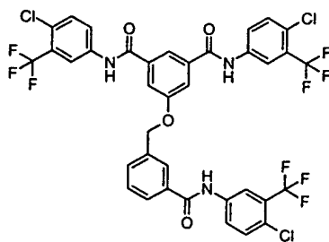
Compound # 37
